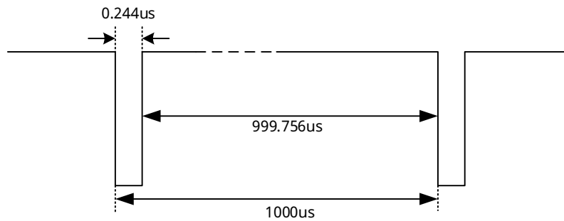
Fig.11 PWM output waveform when PWM_POL=1
