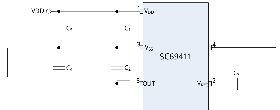
Fig.32 SIP3 Single Chip Reference Circuit Diagram
